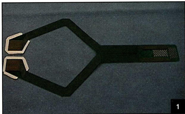
Figure 1. K-scan thin film pressure transducer used to measure contact forces across the medial compartment.
